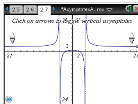
Graph of f(x) = (2x^2-8)/(x^2-16) with asymptotes toggled ON.
