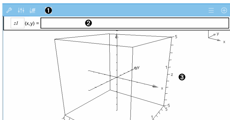
1 3D-Graphen-Symboleiste
